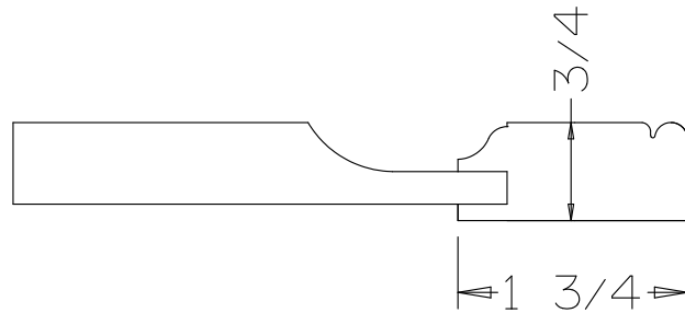
DRAWER FRONT CROSS SECTION
