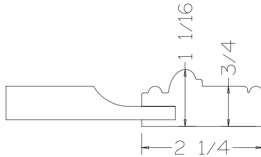
DRAWER FRONT CROSS SECTION
