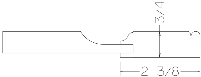
DRAWER FRONT CROSS SECTION
