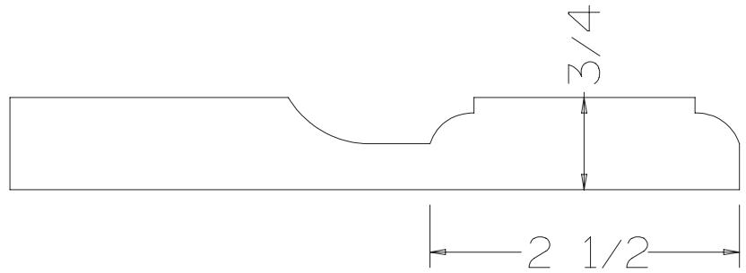
DRAWER FRONT CROSS SECTION
