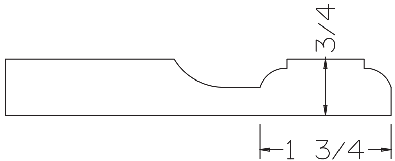
DRAWER FRONT CROSS SECTION
