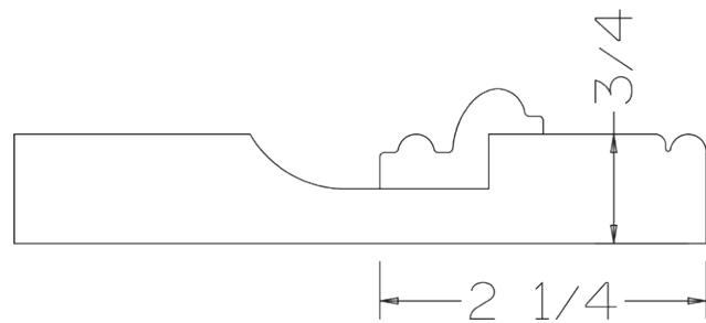
DRAWER FRONT CROSS SECTION
