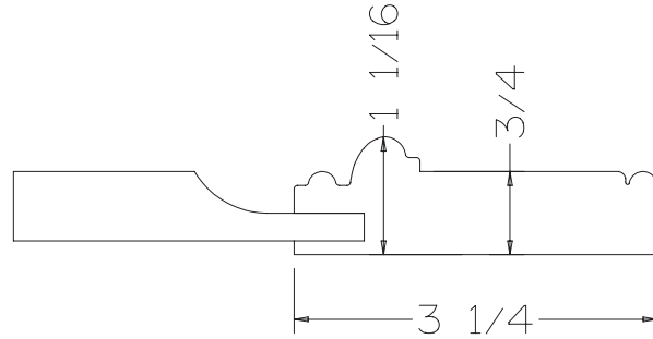
DRAWER FRONT CROSS SECTION
